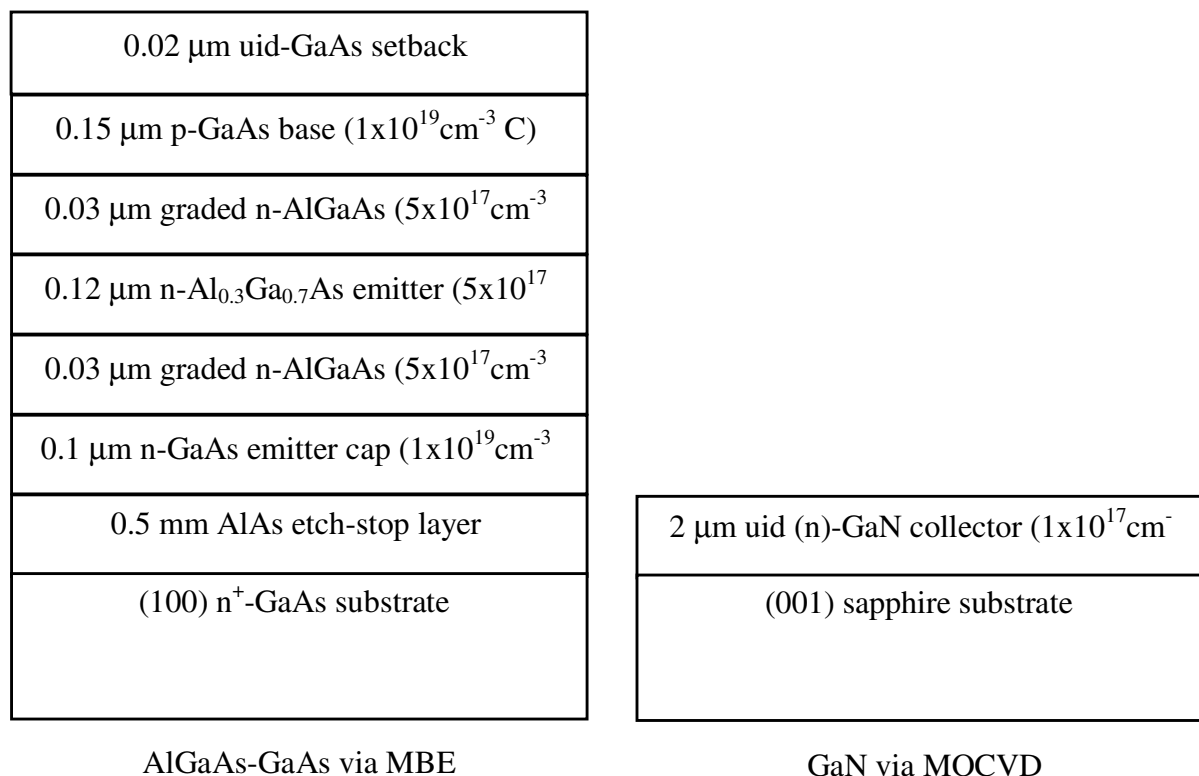
Figure 1. Starting materials for the wafer fusion of the third-generation n-AlGaAs/p-GaAs/n-GaN HBT. In the formation of the HBT, the GaAs and GaN top surfaces are fused together, and then the GaAs substrate and AlAs etch-stop layer are sequentially removed.
