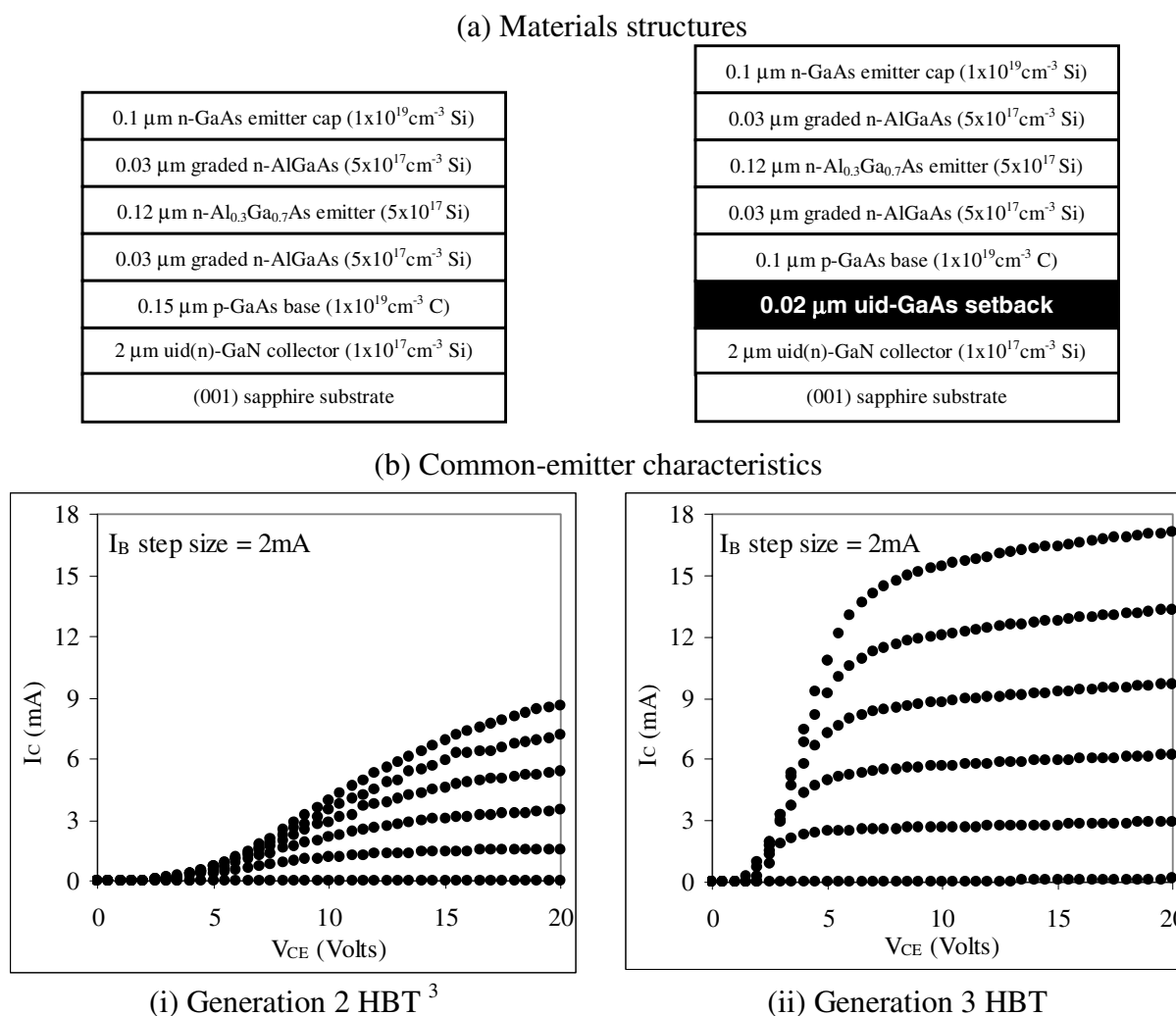
Figure 2. (a) Materials structures and (b) common-emitter characteristics of (i) Generation 2 and (ii) Generation 3 HBTs fused at 600°C. Generation 2 HBTs have no base-collector setback layer and have a thicker base.
